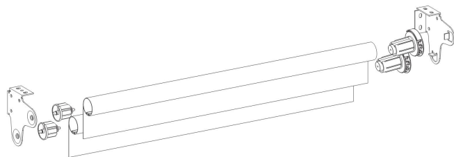
R-001-36A Inner Diameter=36mm Head rail 36铝管 Aluminium Any length available
