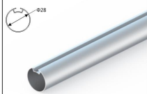
R-001-28A Inner Diameter=28mm Head rail 28铝管 Aluminium Any length available
